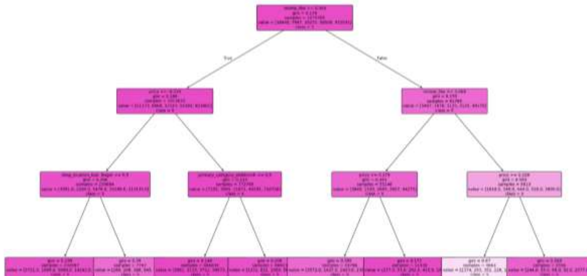
Gambar 2 Decision Tree
